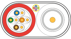
DLC 141 OF + DC power + Coax
