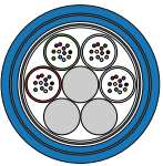
Firetuff LT NM Dielectric, Multitube
