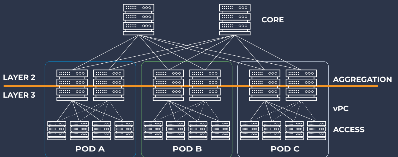
Traditional three-tier data centre design
