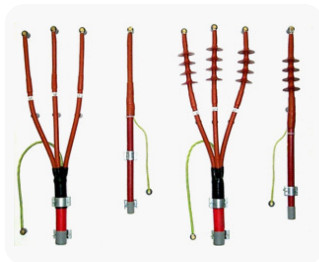
Special sealing end termination for connection box.
